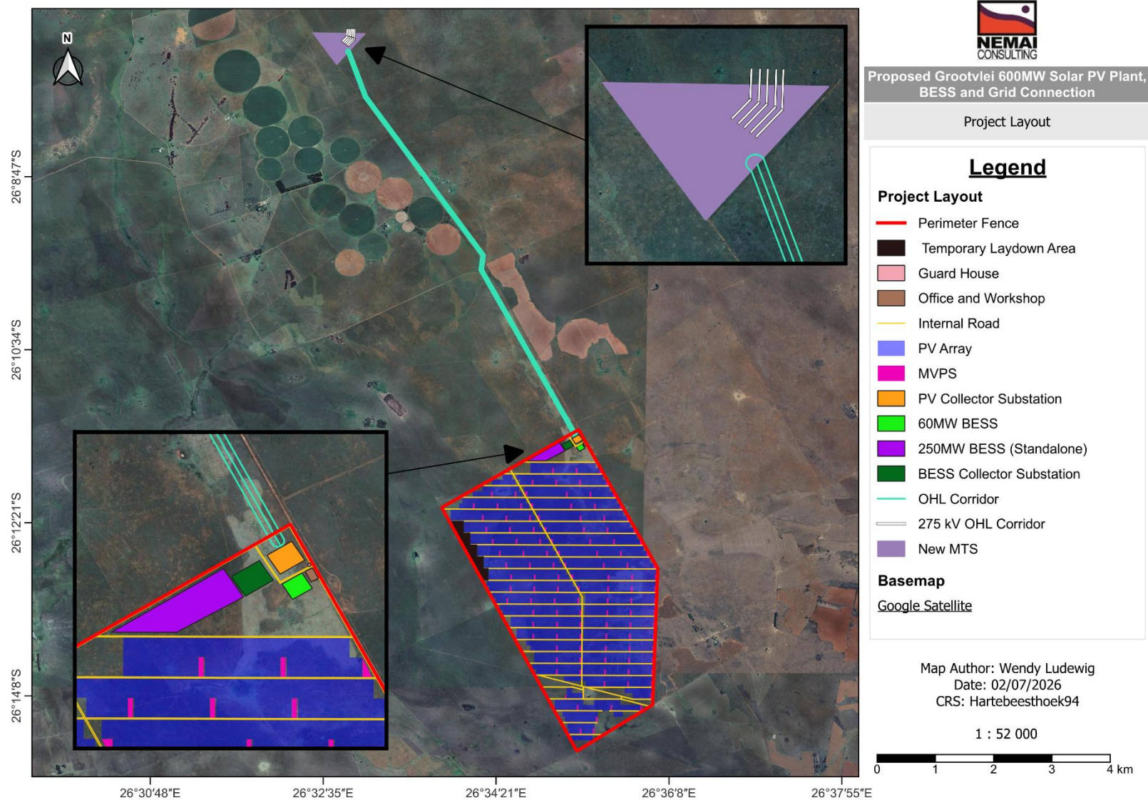
Figure 4: Project Components Layout
